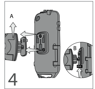
4 Snap the case onto the bracket.
