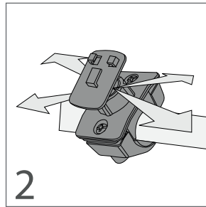
2 Adjust the tilt of the base as desired.
